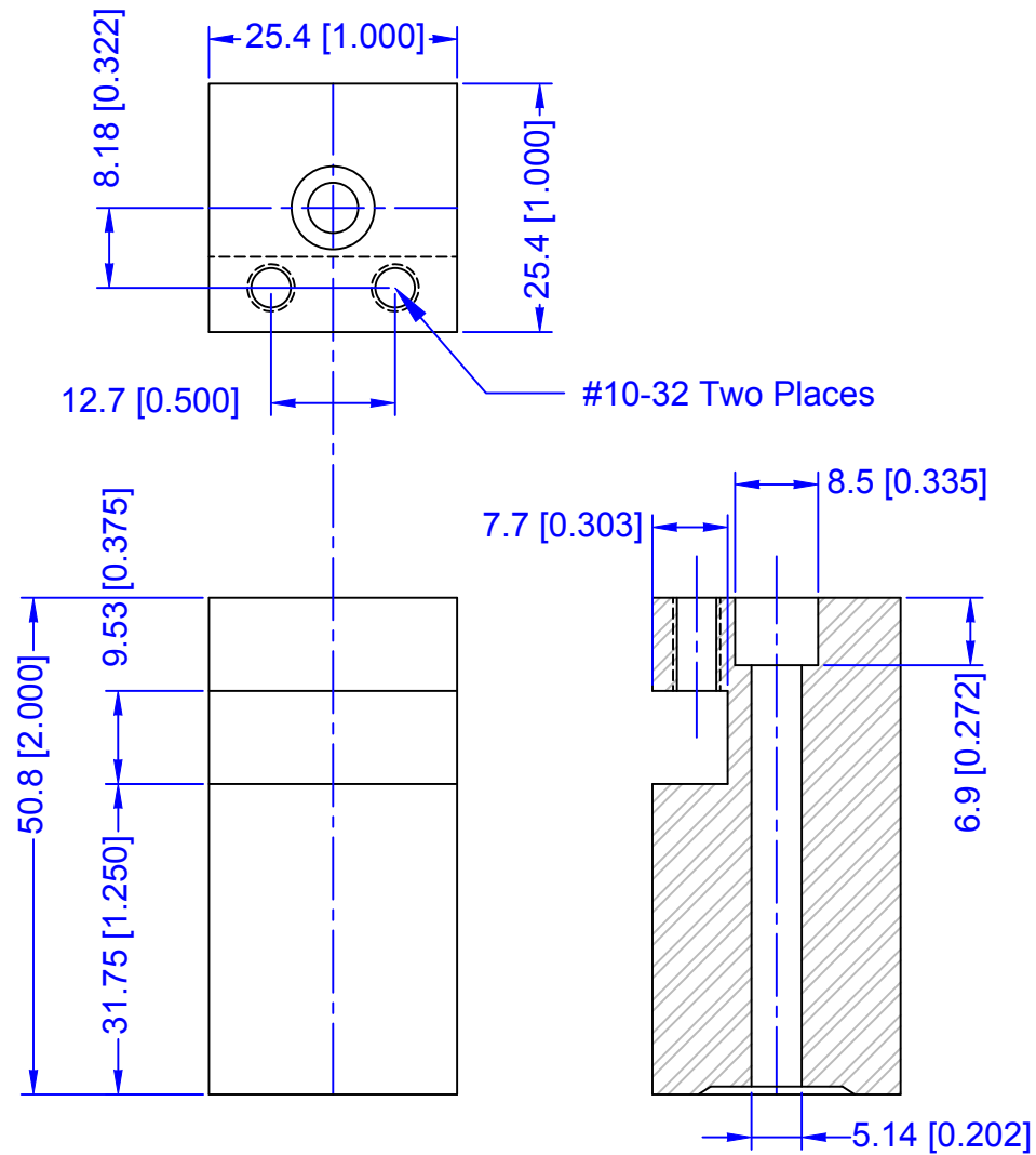
Taig Standard Back Tool Post
