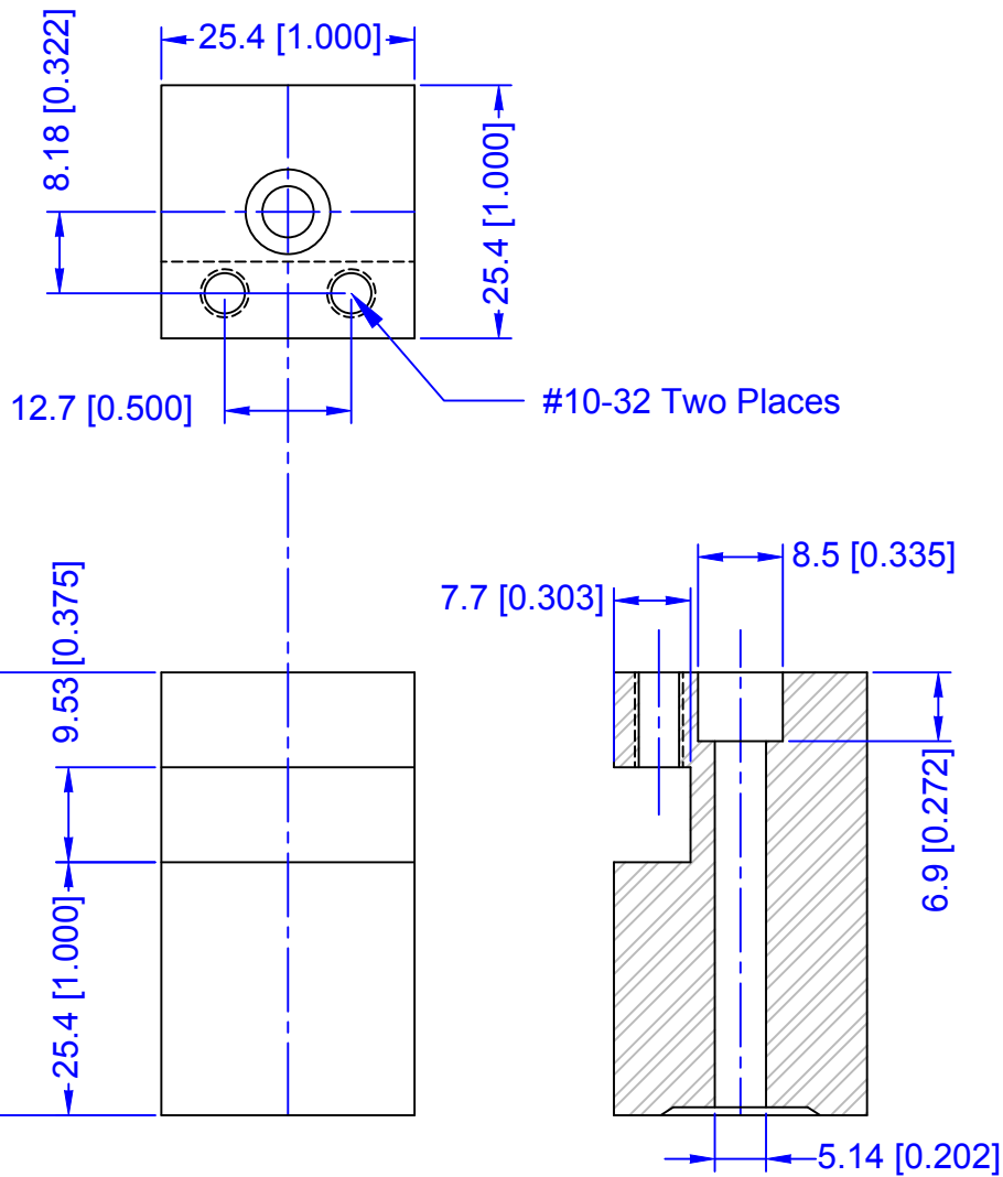
Taig Standard Front Tool Post
